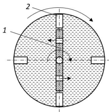
Figure 4. – Rotational dashpot
