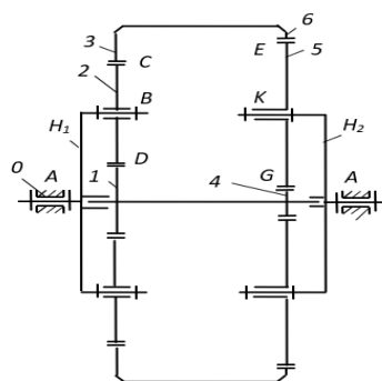
Figure 3. – Initial kinematic chain ssg
