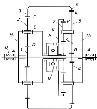
Figure 1. – Stepless self-controlled gearbox (ssg)
